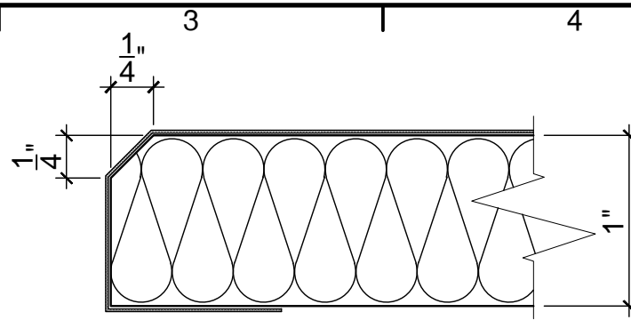
1/4" BEVEL
